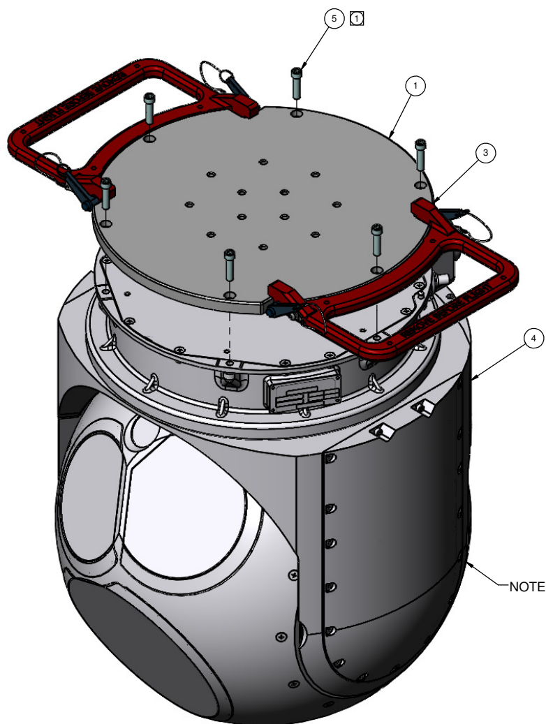
EXPLODED PARTS VIEW
