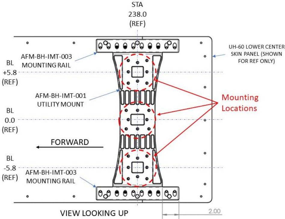
Figure 12. Lateral Mounting Locations – AFM-BH-IMT-1 I-Mount
