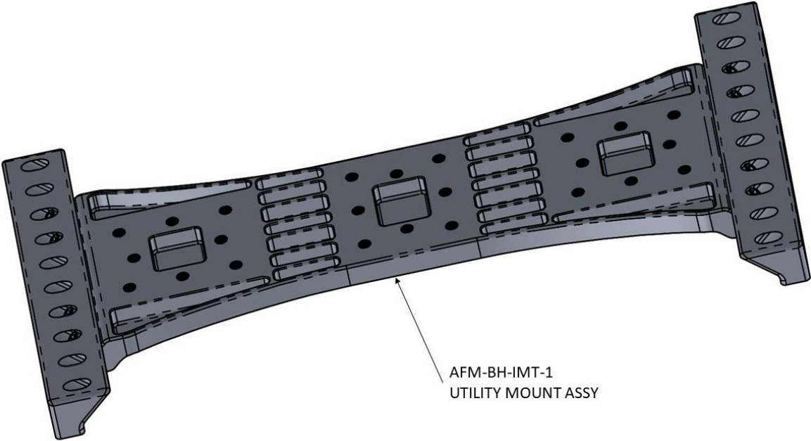
Figure 6. Assembled View of AFM-BH-IMT-1 I-Mount (CAD Illustration)
