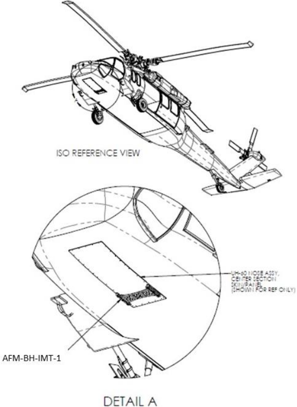
Figure 3. CAD Illustration View Showing AF-BH-IMT-1 Installation on a UH-60 Helicopter
