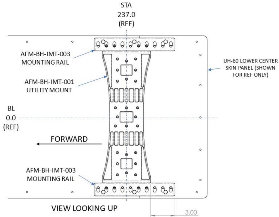
Figure 10. Configuration #4 – AFM-BH-IMT-1 I-Mount, Forward/Center Position
