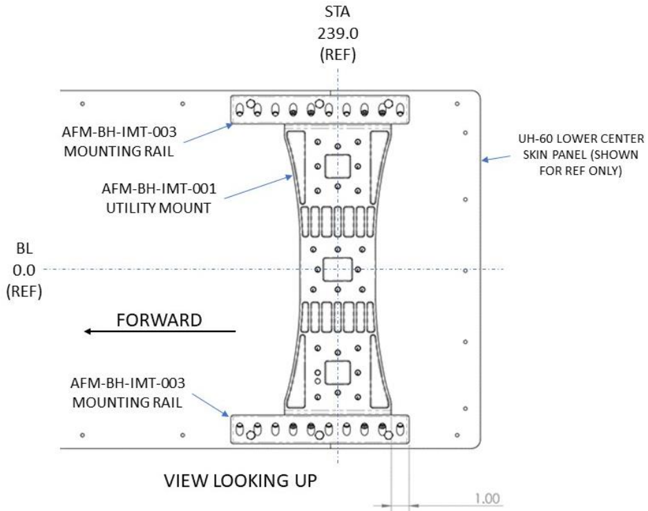
Figure 8. Configuration #2 – AFM-BH-IMT-1 I-Mount, Aft/Center Position
