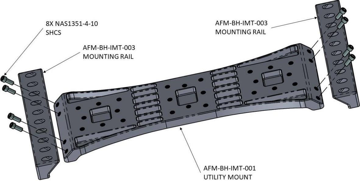
Figure 5. Exploded Assembly View of AFM-BH-IMT-1 I-Mount (CAD Illustration)
