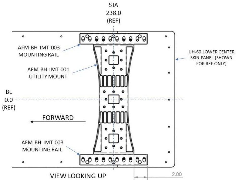
Figure 9. Configuration #3 – AFM-BH-IMT-1 I-Mount, Center Position
