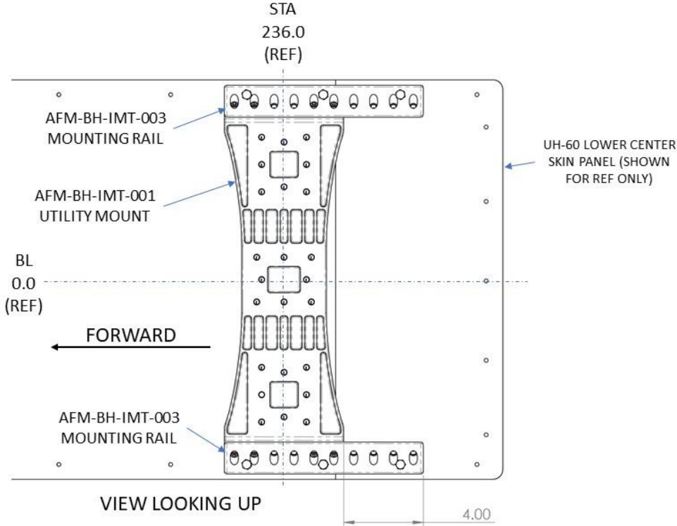
Figure 11. Configuration #5 – AFM-BH-IMT-1 I-Mount, Forward Position
