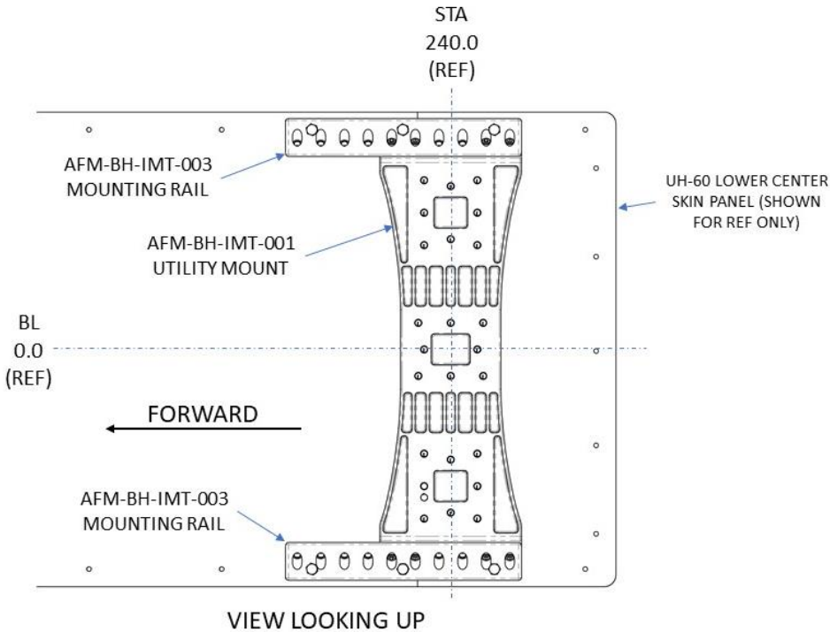
Figure 7. Configuration #1 – AFM-BH-IMT-1 I-Mount, Aft Position
