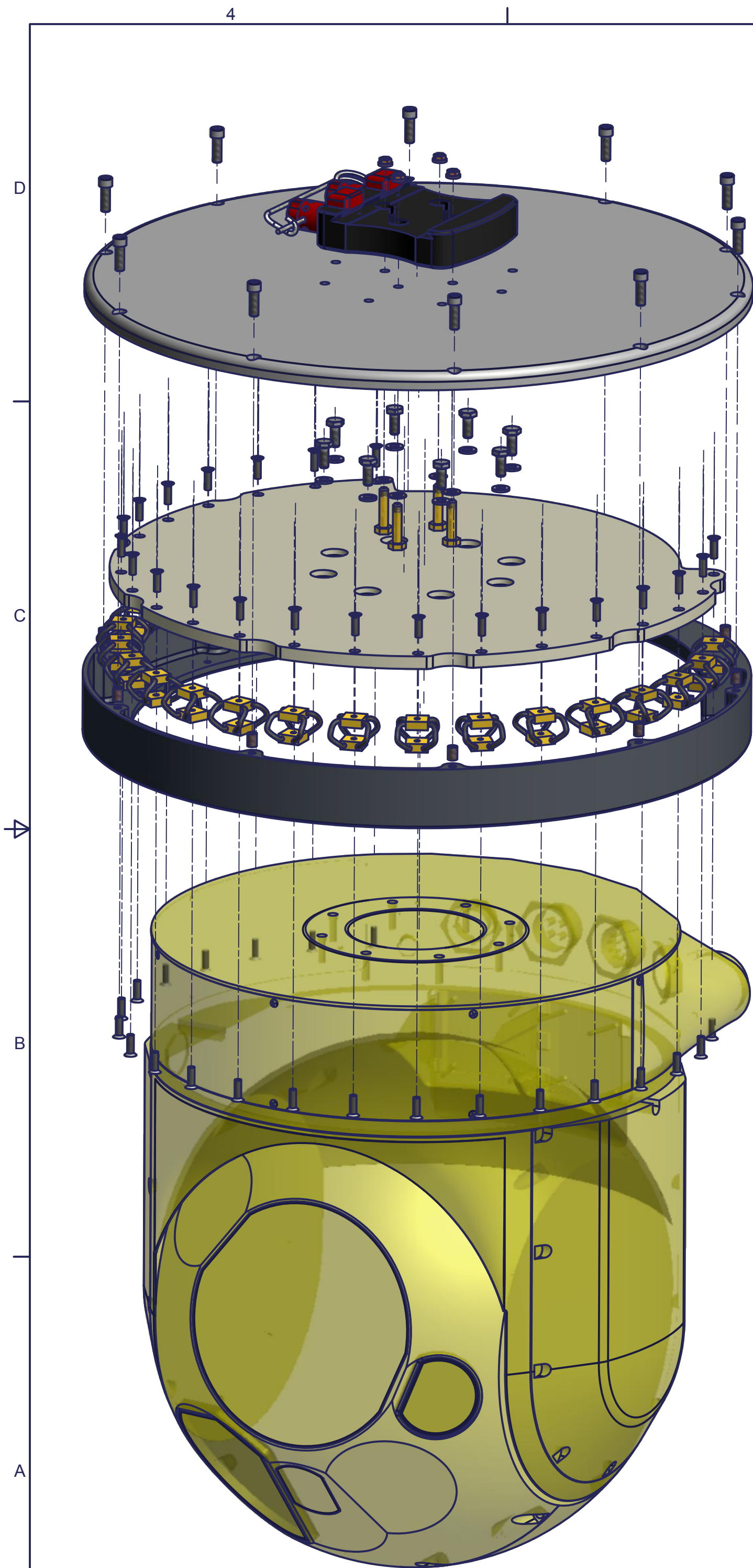
AUX EXPLODED VIEW
